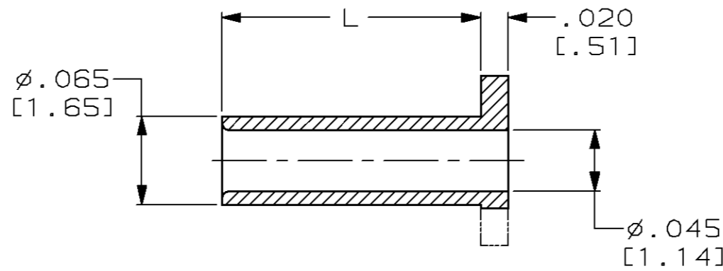
SECTION Z-Z
